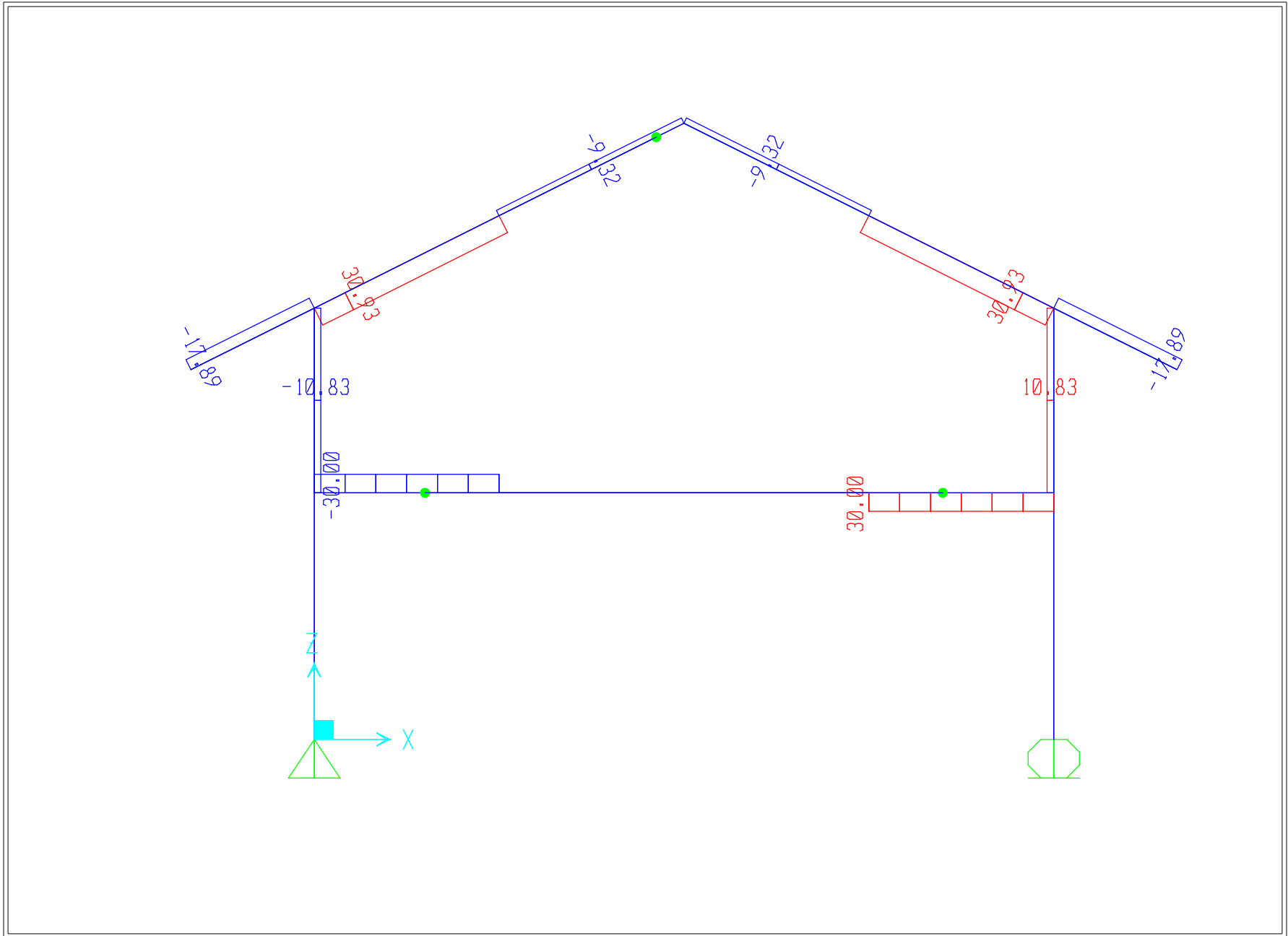
SAP2000 v15.1.0 - File:18 - Shear Force 2-2 Diagram (DEAD) - KN, m, C Units
